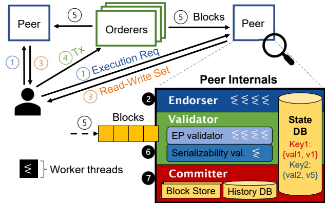
Figure 1: Transaction flow and peer internals
