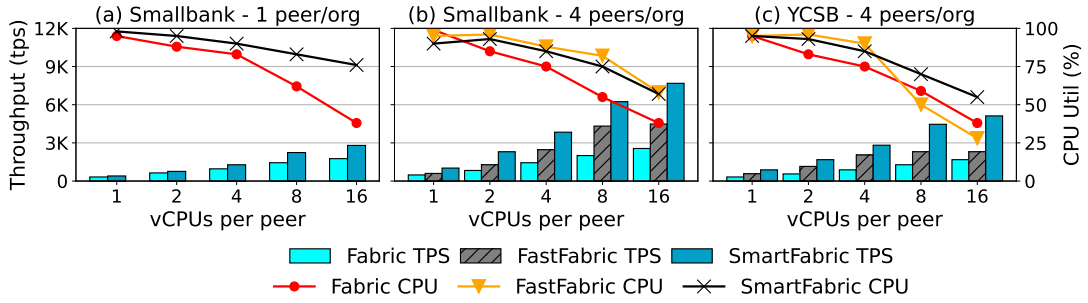
Figure 9: Vertical Scaling
