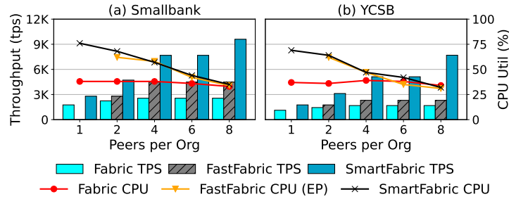
Figure 10: Horizontal Scaling
