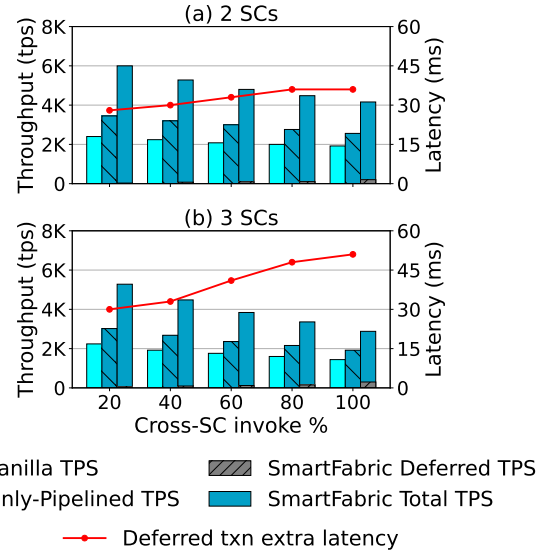
Figure 15: Cross-contract transactions
