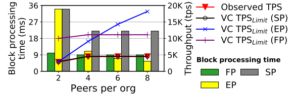
Figure 12: FastFabric’s block processing time
