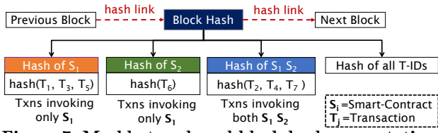
Figure 7: Merkle tree based block hash computation.
