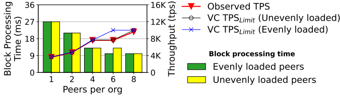
Figure 11: Effect of imbalanced load on Sparse Peers
