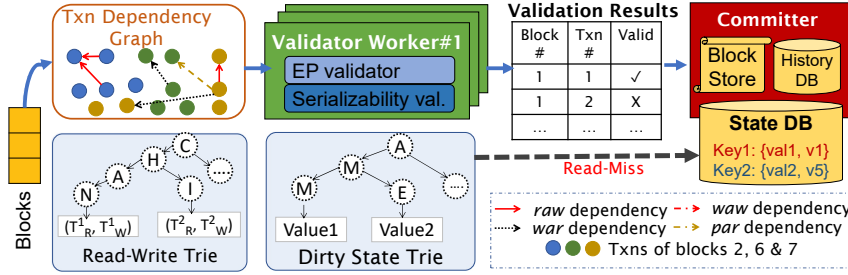
Figure 5: Components involved in pipelined validation and commit
