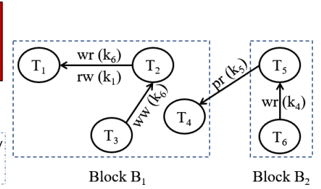
Figure 6: Example dependency graph
