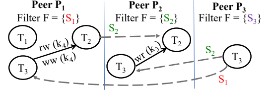
Figure 8: Tx. dependency graphs
